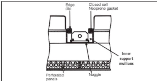
Multi-panel unit frame details surface mounting
